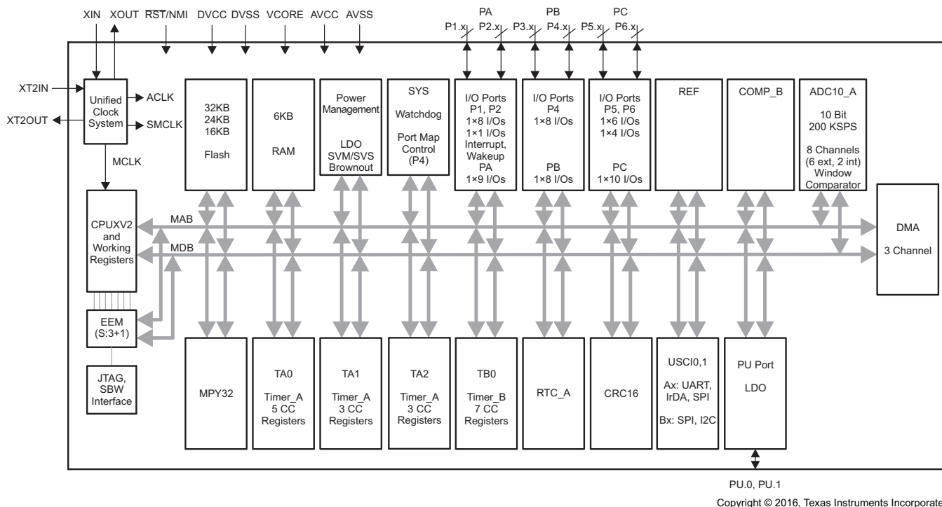
Figure 1-2. Functional Block Diagram – MSP430F5310IRGZ, MSP430F5309IRGZ, MSP430F5308IRGZ, MSP430F5310IPT, MSP430F5309IPT, MSP430F5308IPT
