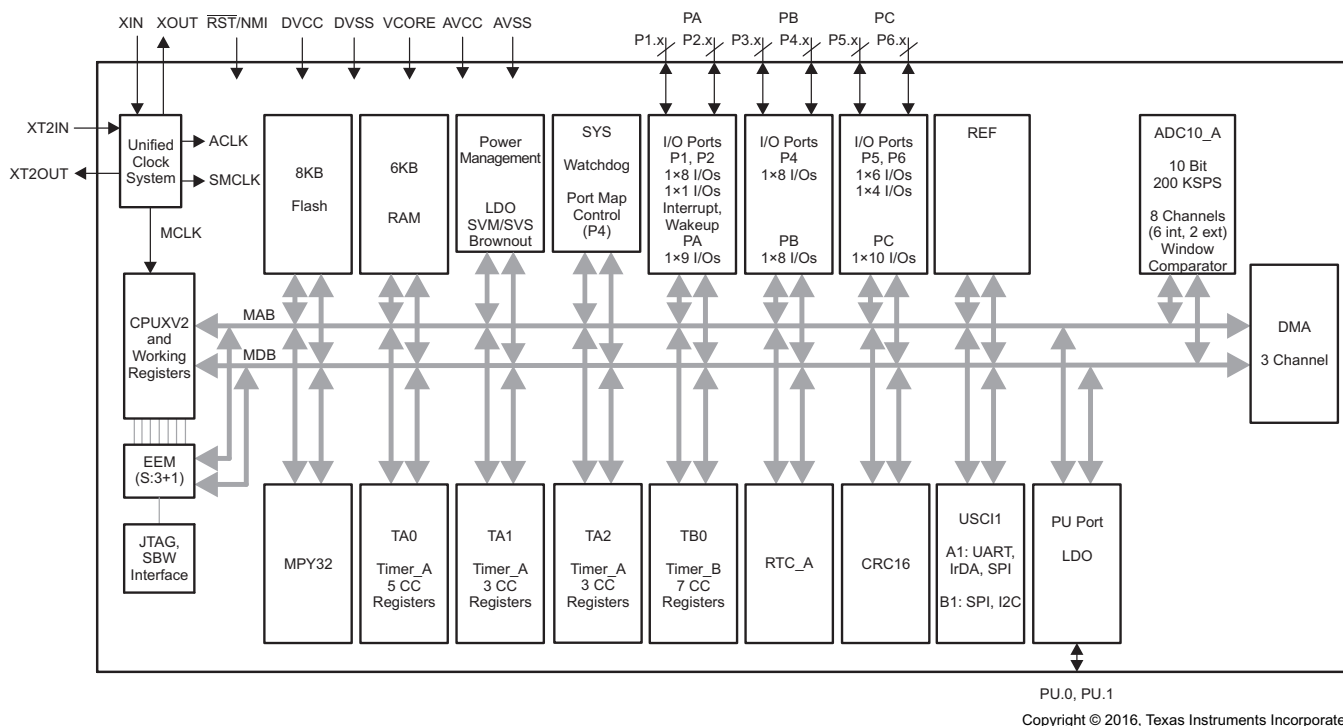
Figure 1-3. Functional Block Diagram – MSP430F5304IRGZ, MSP430F5304IPT
